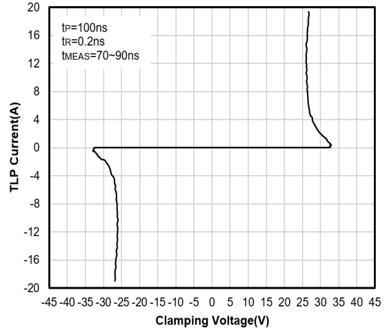
TLP Curve
